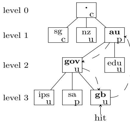
(a) Inherited Poison
