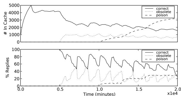
4: Evolution of a Standard DNS Cache
