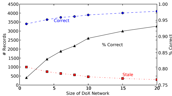
6: Improving Cache Consistency
