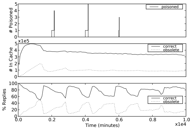
5: Poison Detection and Removal
